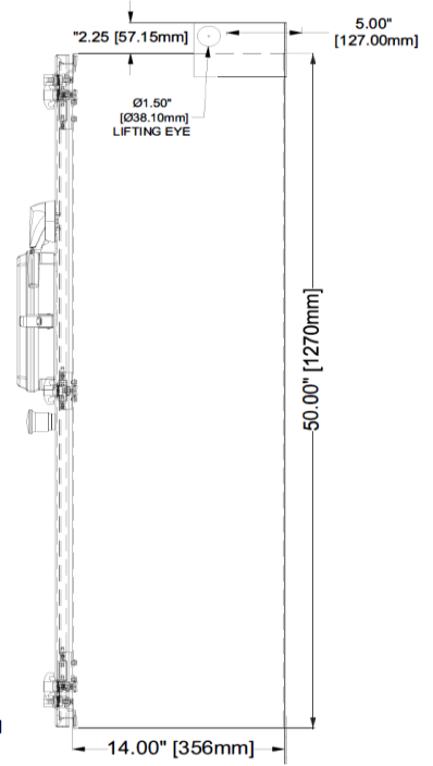
RHS VIEW
