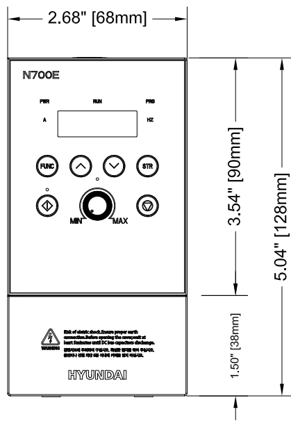
FRONT (FACE)
