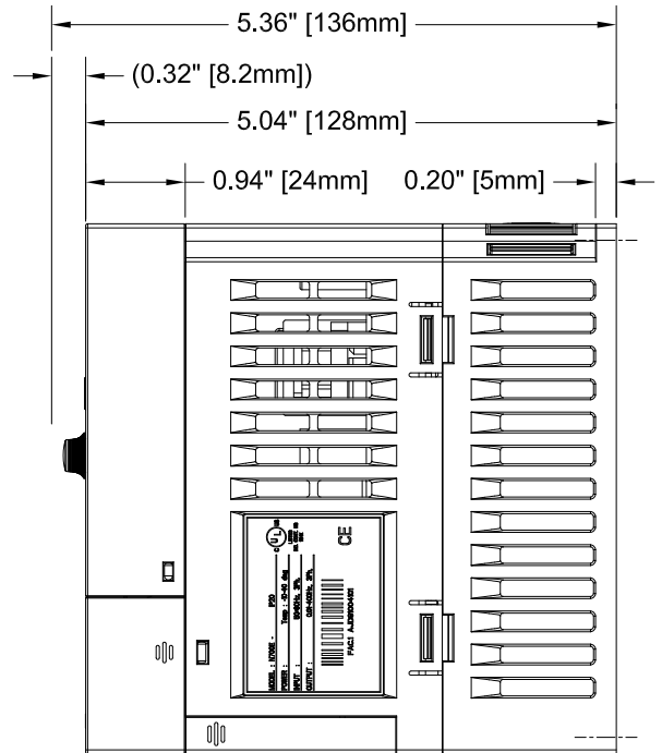
RH SIDE
