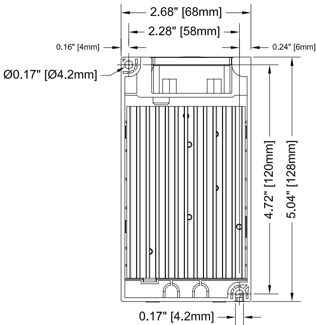
UNDERSIDE
