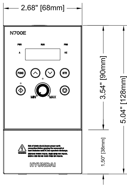
FRONT (FACE)
