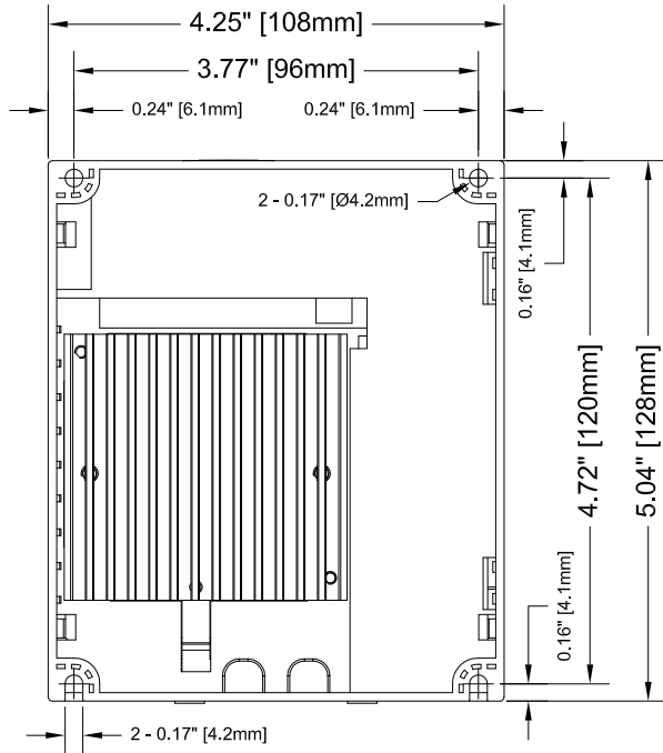
UNDERSIDE
