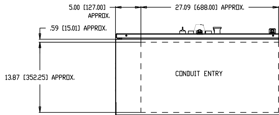
BOTTOM VIEW
