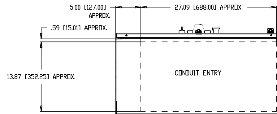
BOTTOM VIEW
