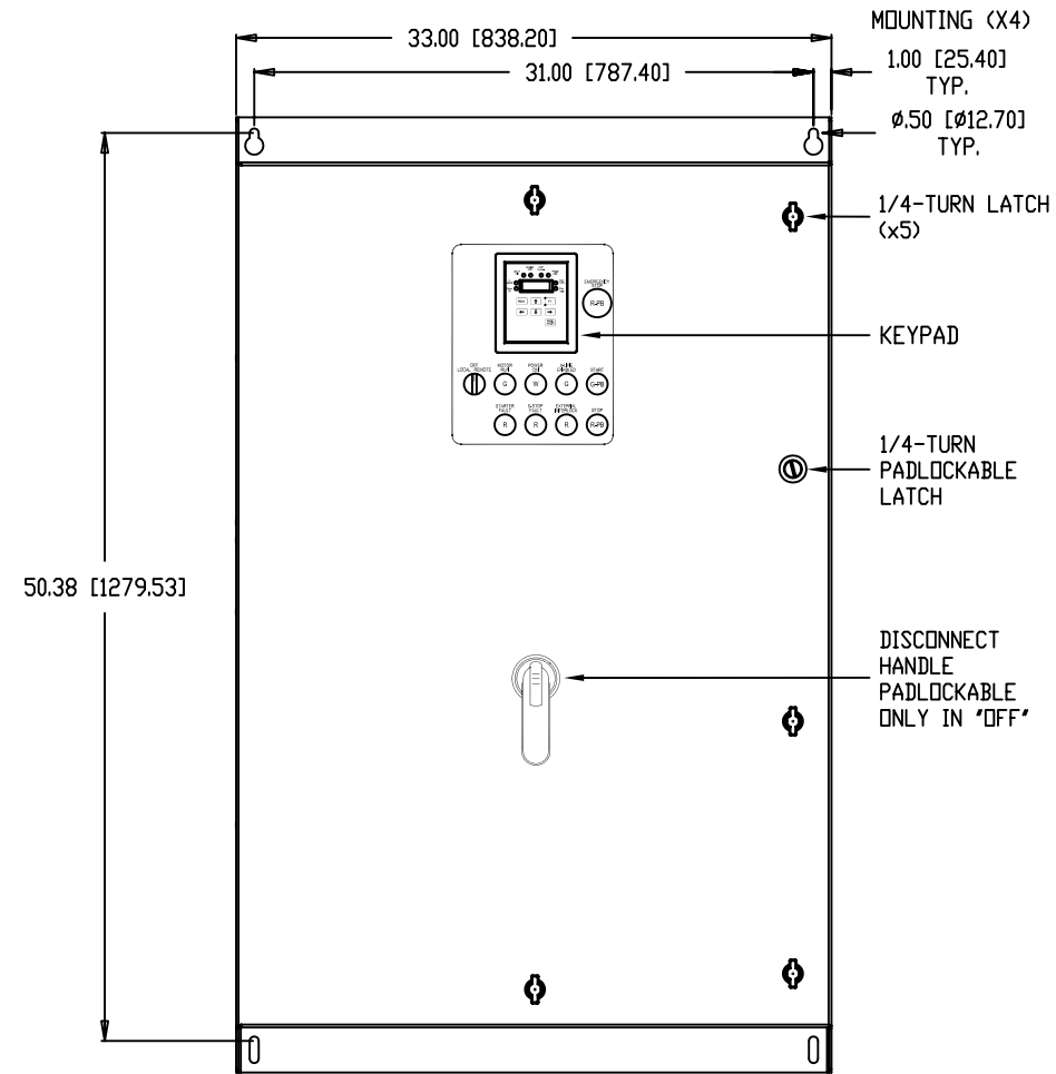
FRONT VIEW
