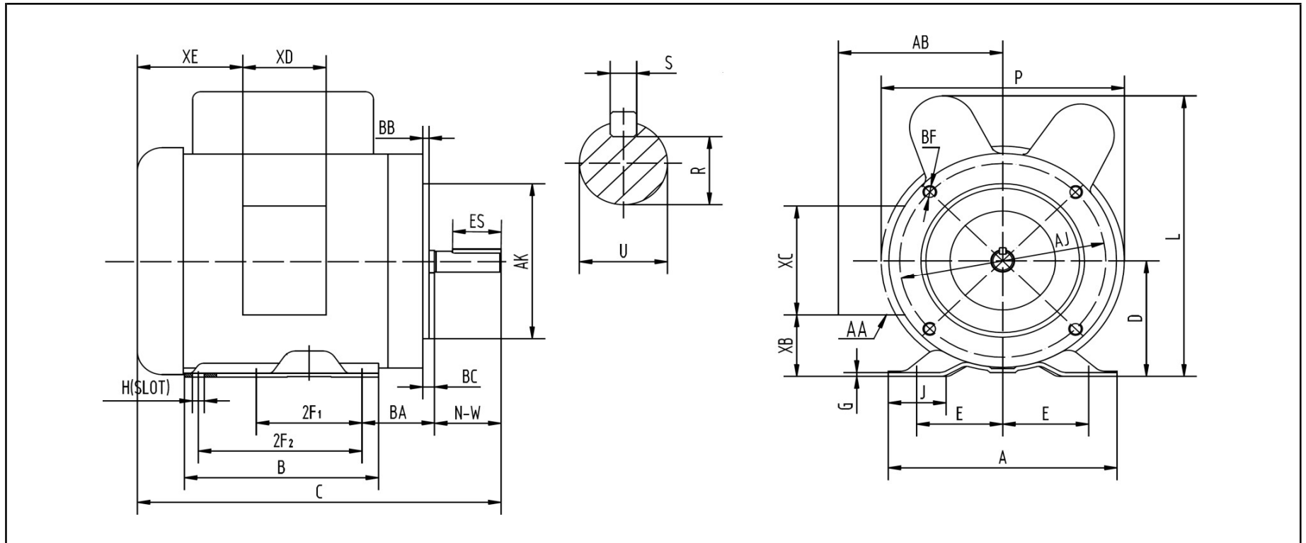
DIMENSIONS - INCHES
