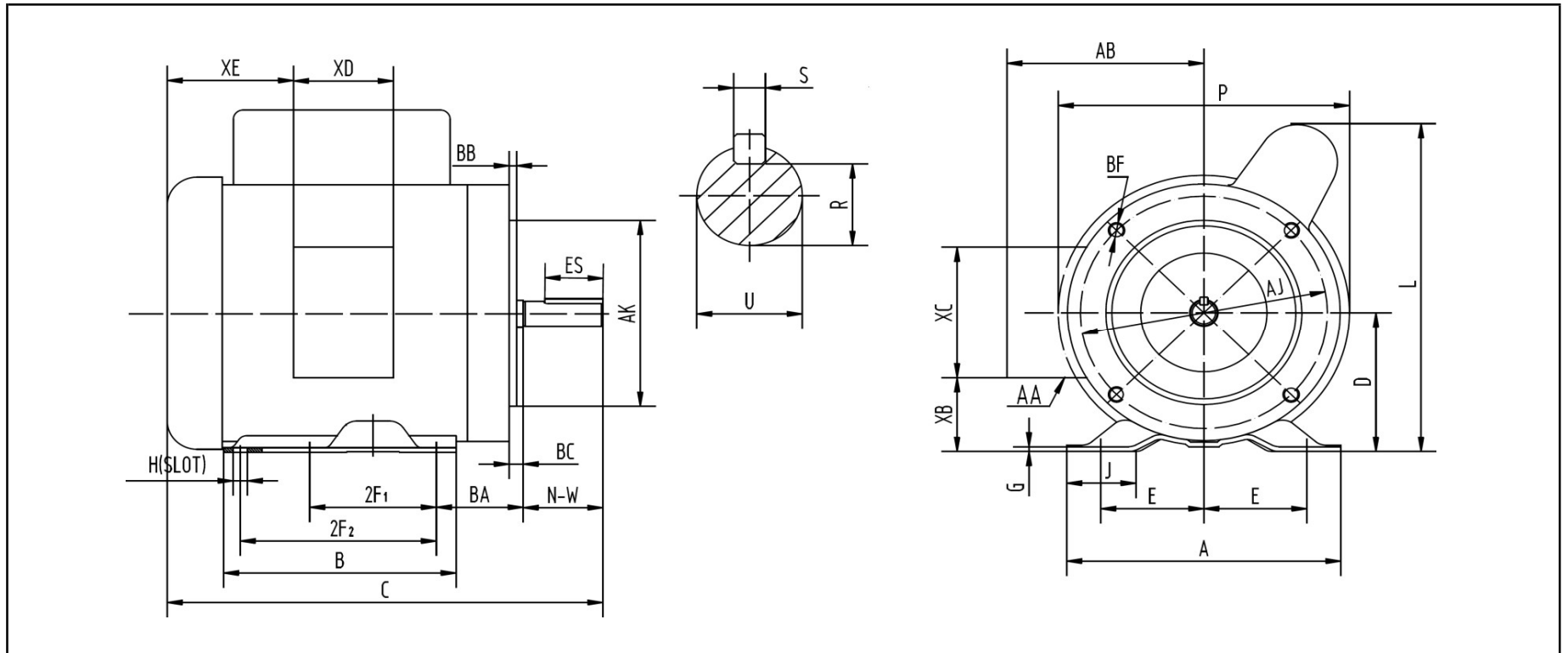
DIMENSIONS - INCHES
