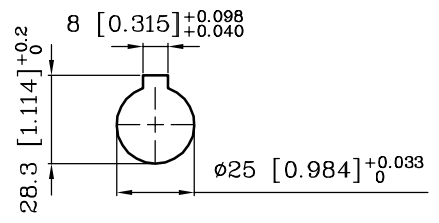
OUTPUT BORE
