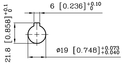
INPUT BORE
