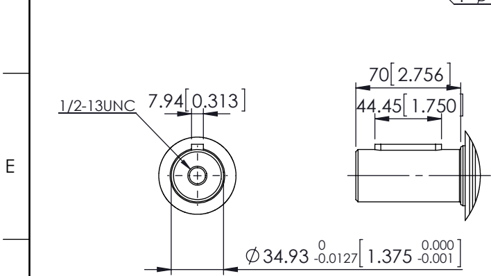
OUTPUT SHAFT
